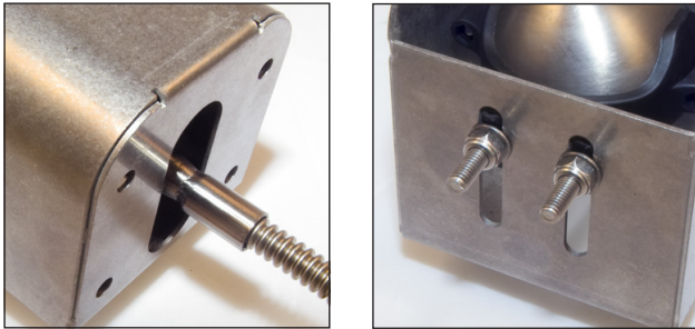
Slotting holes for positioning camera in vertical and horizontal direction.
